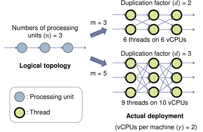
Figure 4. Examples of scaling a topology with three processing units ( n = 3 ) to three and five machines ( m = 3 and 5 ) respectively. Each machine has two vCPUs ( \gamma = 2 ).
