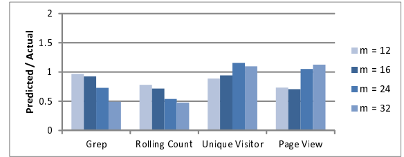
Figure 7. Normalized prediction accuracy obtained from Model 1.
